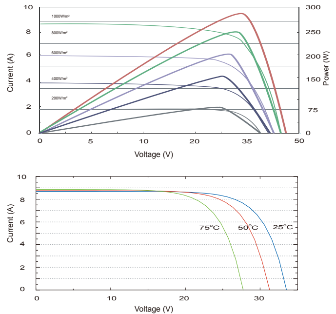
Current-Voltage & Power-Voltage Curves (280W)
