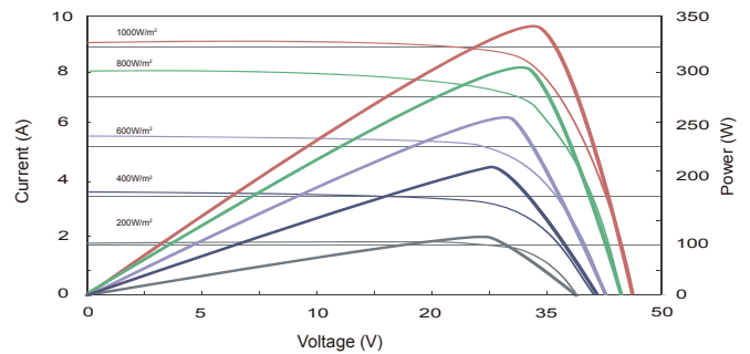
Current-Voltage & Power-Voltage Curves (340W)
